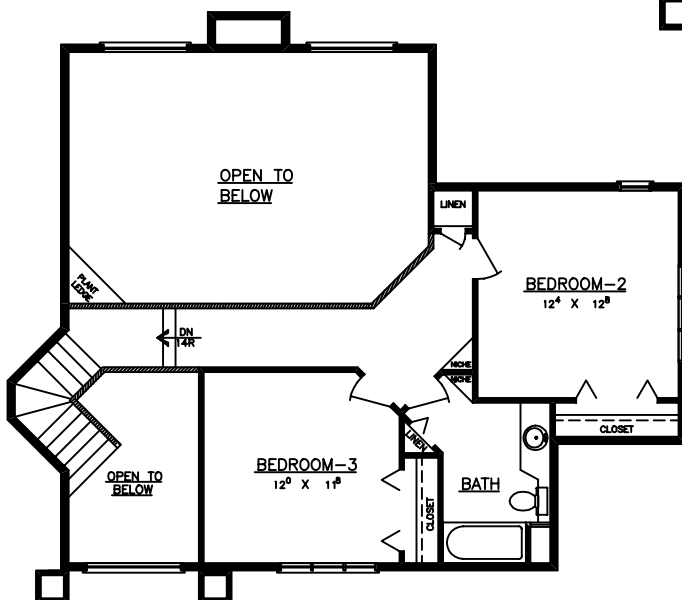
SECOND FLOOR
